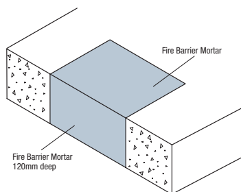
Concrete Floor 120mm – FRL: -/180/180
