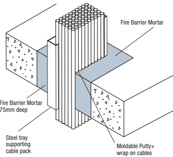
Concrete Floor 120mm – FRL: -/120/-
